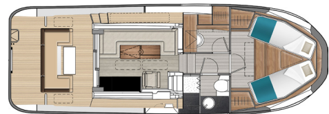
Lower deck - 1 cabin / 1 head
